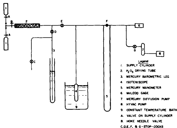
Fig. 1. Low-vapor-pressure equipment.
